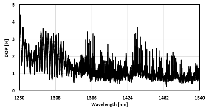
FIG. 10: DEGREE OF POLARIZATION
