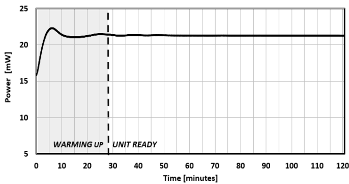
FIG. 9: WARM-UP TIME
