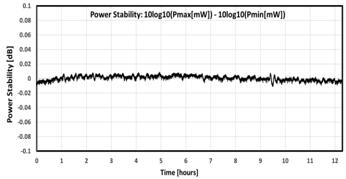
FIG. 8: ISB2 TYPICAL POWER STABILITY
