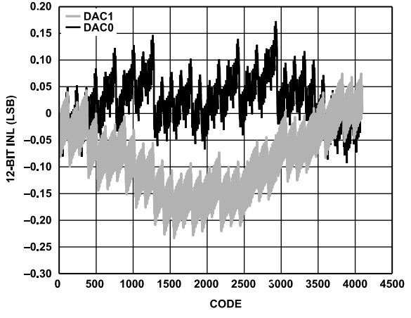
Figure 38. INL, I_{OUTFS} = 20\text{ mA} , 12-Bit Resolution
