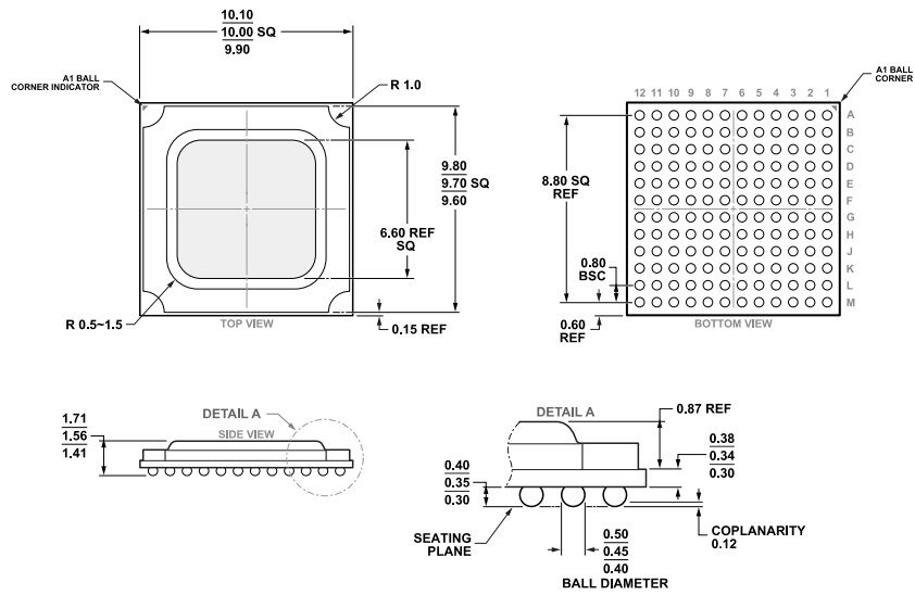
Figure 86. 144-Ball Ball Grid Array, Thermally Enhanced [BGA_ED] (BP-144-1) Dimensions shown in millimeters
