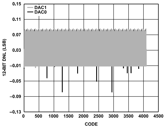
Figure 37. DNL, I_{OUTFS} = 20\text{ mA} , 12-Bit Resolution
