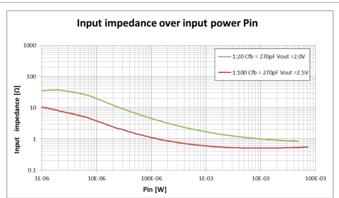
Figure 5-8 Input Impedance vs Power C FB 270 pF
