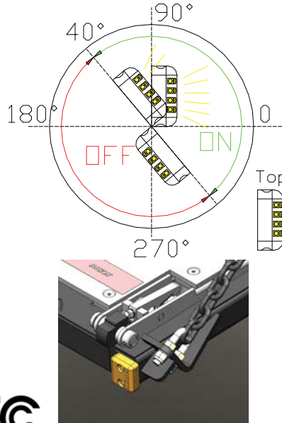
Recommened Mounting position
