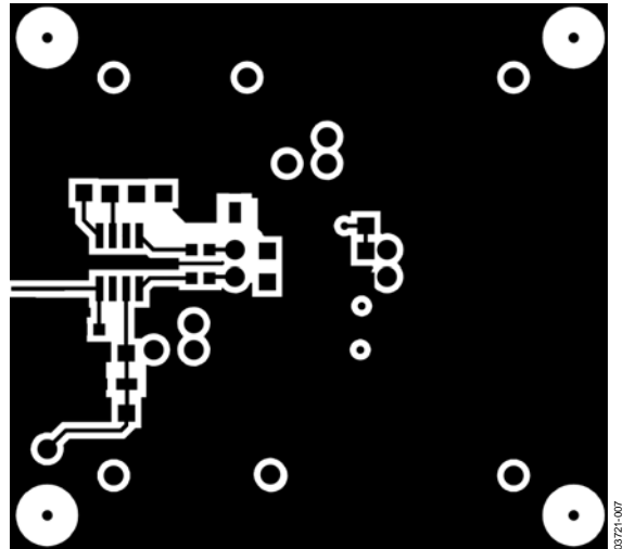
Figure 8. Wiring-Side Pattern
