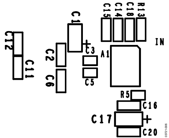
Figure 7. Wiring-Side Silkscreen
