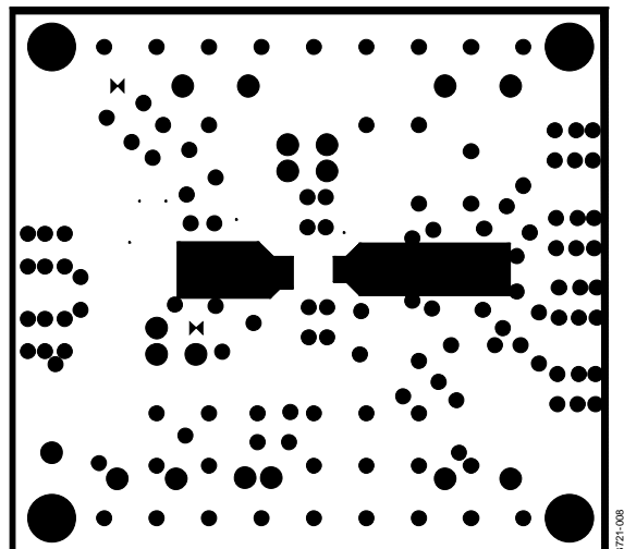
Figure 9. Inner Layer 2
