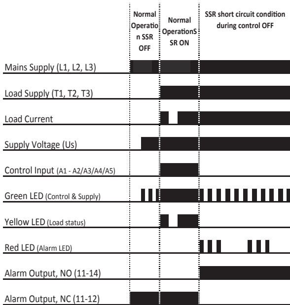
Operation diagram 5
