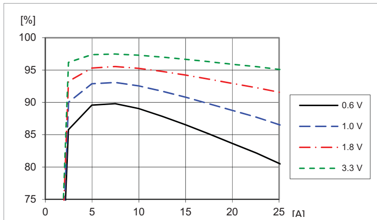
Efficiency vs. Output Current, V_I = 5\text{ V}
