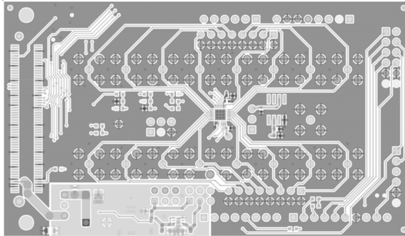
Figure 11. EVAL-AD5677RSDZ Top Side Routing
