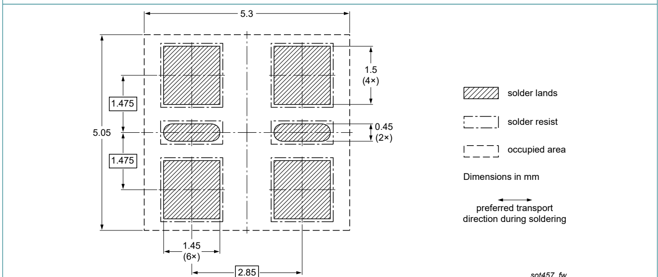
Fig. 10. Wave soldering footprint for SC-74; TSOP6 (SOT457)
