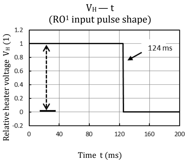
Relative rectangular heater voltage (V H ) pulse with a relative pulse width of 124 ms at 5 Hz (time description of reference operation RO 1 )
