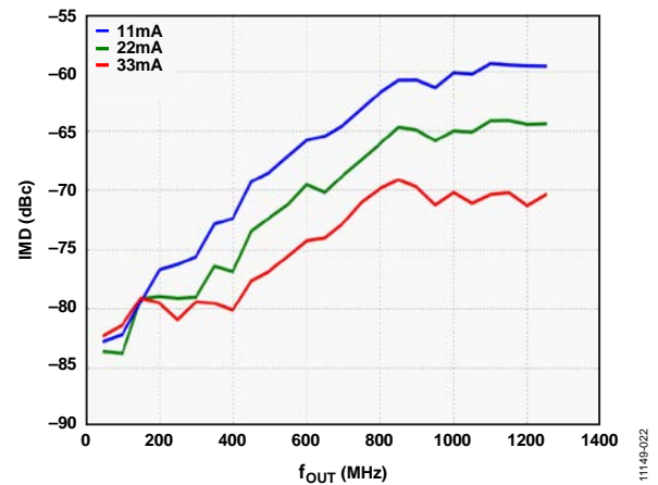
Figure 19. IMD vs. f_{OUT} over DAC I_{OUTFS}
