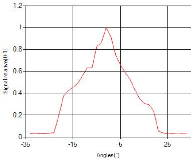
Radiation Distribution
