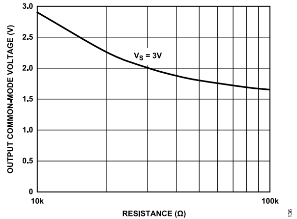
Figure 38. Output Common-Mode Voltage vs. R_{CM} to COMM
