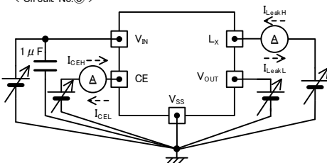
< Circuit No.⑤ >
