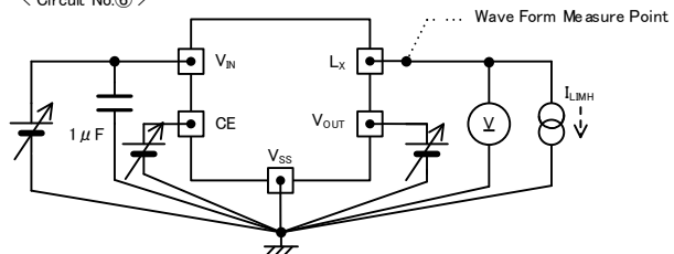
< Circuit No.⑥ >
