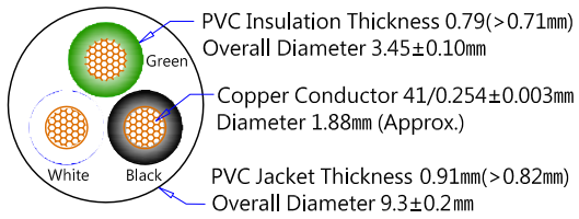
SJT 14AWGx3C截面圖 (Wire Cross-Section)
