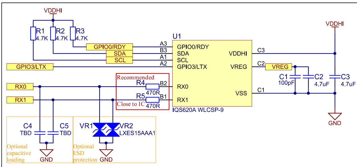
Figure 1.5 IQS620A WLCSP-9 reference schematic
