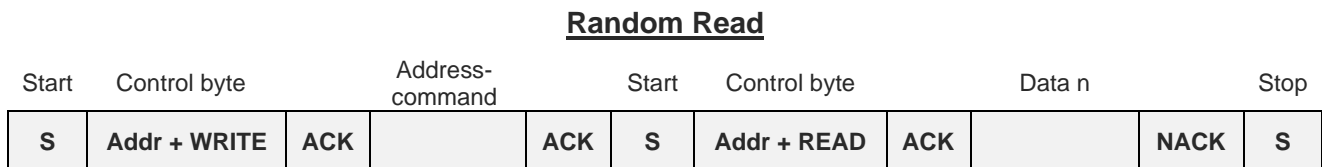
Figure 7.2 Random Read
