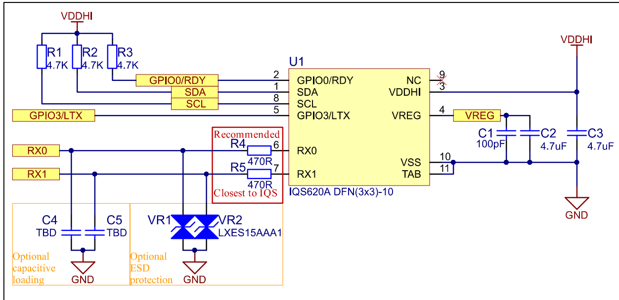
Figure 1.4 IQS620A DFN(3x3)-10 reference schematic
