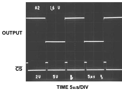
Figure 14. Large Signal Settling Time
