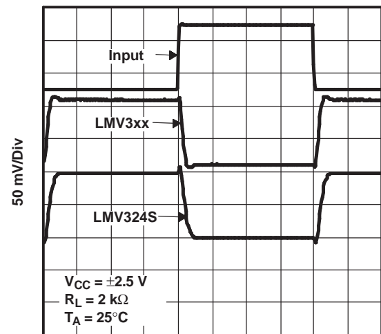
1 μs/Div Figure 36.
