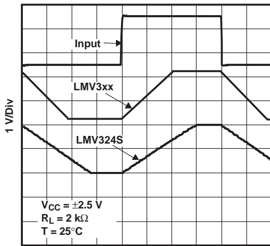
1 \mu\text{s}/\text{Div} Figure 27.
