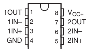
LMV358 . . . D (SOIC), DDU (VSSOP), DGK (MSOP), OR PW (TSSOP) PACKAGE (TOP VIEW)
