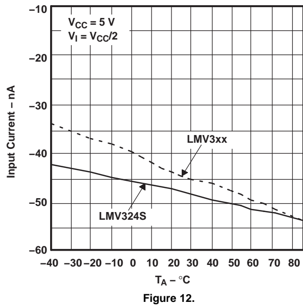
INPUT CURRENT vs TEMPERATURE
