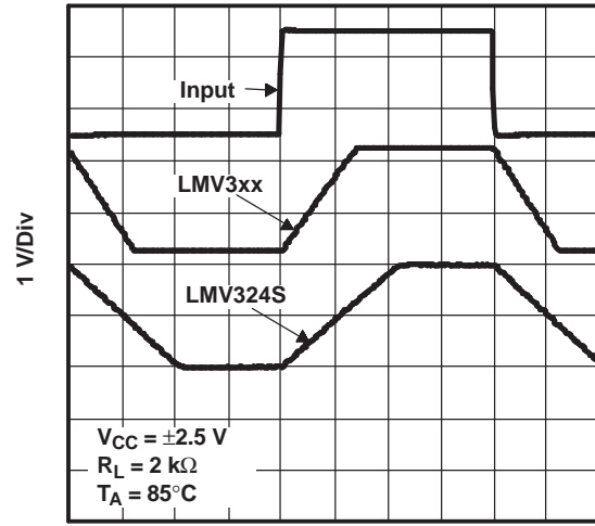
1 \mu\text{s}/\text{Div} Figure 28.
