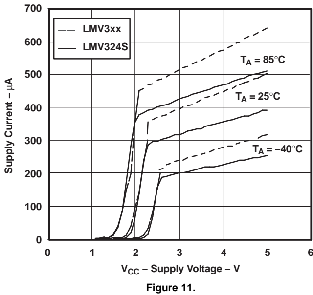
SUPPLY CURRENT vs SUPPLY VOLTAGE – QUAD AMPLIFIER
