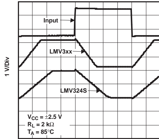
1 μs/Div Figure 34.
