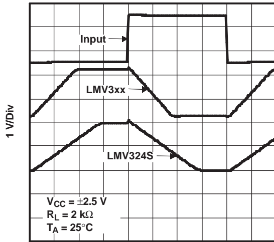
1 μs/Div Figure 33.
