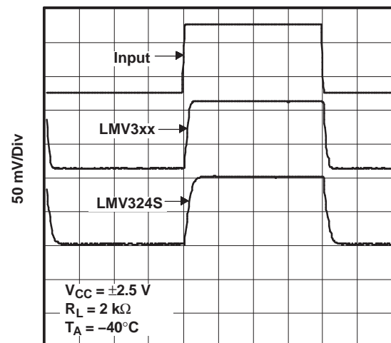
1 \mu\text{s}/\text{Div} Figure 32.
