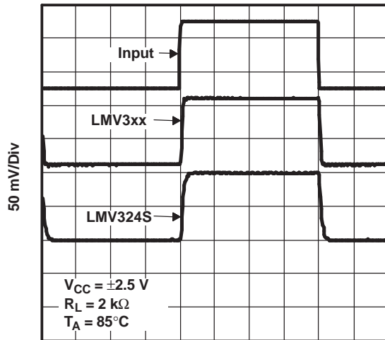
1 \mu\text{s}/\text{Div} Figure 31.
