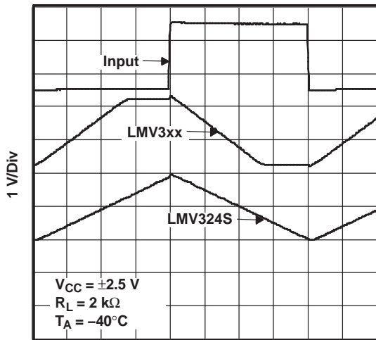
1 μs/Div Figure 35.
