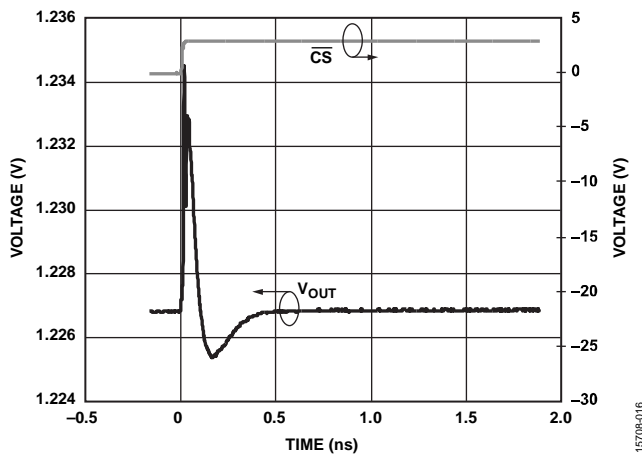
Figure 16. Digital-to-Analog Glitch Impulse
