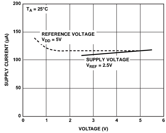
Figure 13. Supply Current vs. Voltage (Reference and Supply)
