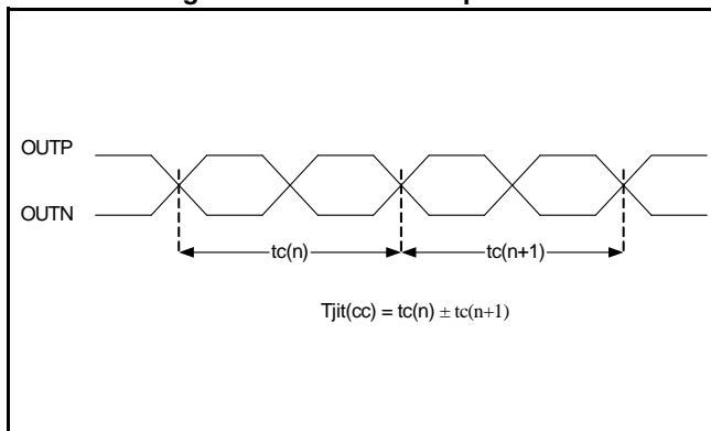
Figure 3: Cycle-cycle jitter
