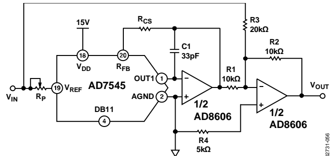
Figure 56. Bipolar Operation
