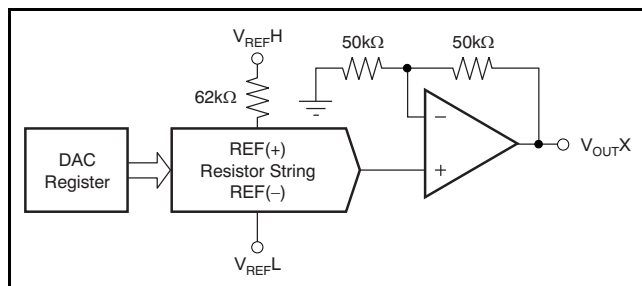
Figure 92. DAC8564 Architecture
