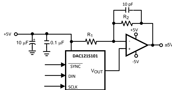
Figure 45. Bipolar Operation
