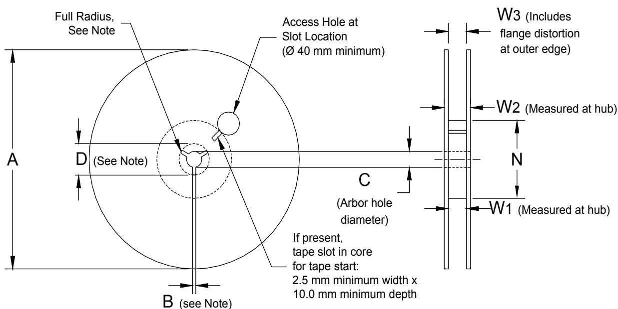
Figure 5 – Reel Dimensions
