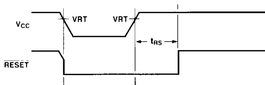
Figure 3. Power Off/On RESET Timing
