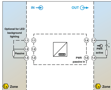
Block diagram FA MCR-EX-DS-I-OLP
