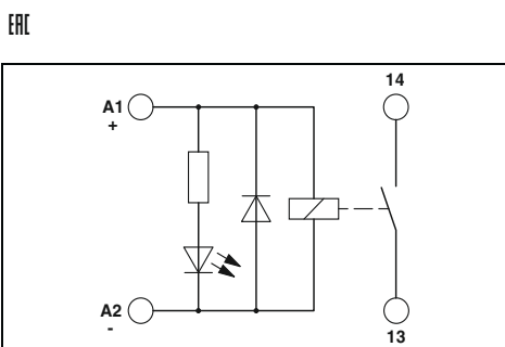
Medium to high powers 1 N/O contact (1)
