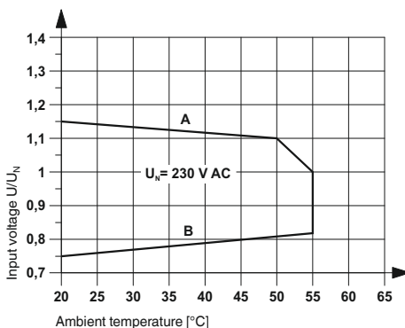
Permissible input voltage range for PLC-RSP-230UC/21-21AU/RWF
