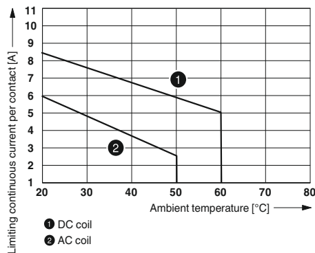
Contact derating
