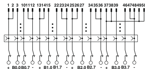
Connection scheme FLKM 50/KDS3-MT/PPA/PLC
