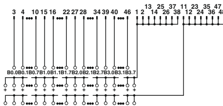
Connection scheme FLKMS 50/32IM/PLC
