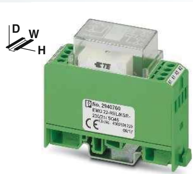
1 changeover contact, soldered-in relay
