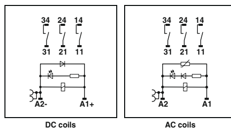
DC coils
