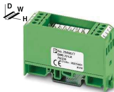
Light indicator module, with common return line
