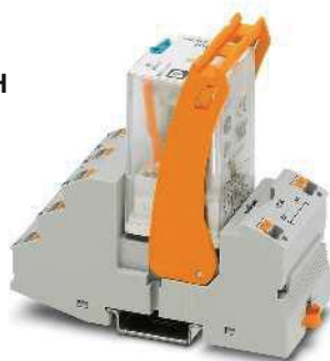
3-changeover-contact octal relay module with Push-in connection and manual operation
