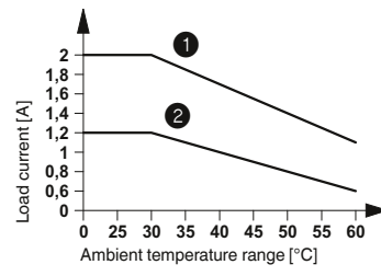
Derating curve for OPT...DC/230AC/2 and PLC-OS.../230AC/2/ACT solid-state relays
