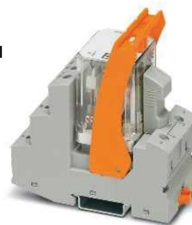
2 changeover-contact high-power relay module with screw connection
