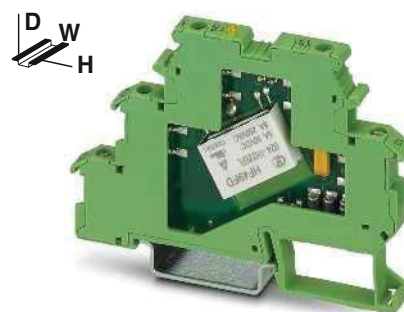
For low to medium powers 1 N/O contact (1)
