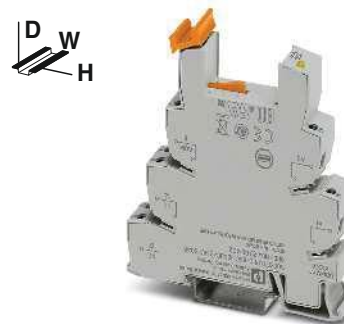
1-changeover-contact basic terminal block for high continuous currents with input filter
