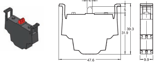
Mounting Latches A22NZ-H-02
