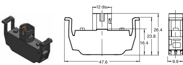
Lighting unit A22NZ-T□PN
