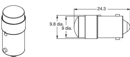
LED Lamp A22NZ-L□□
