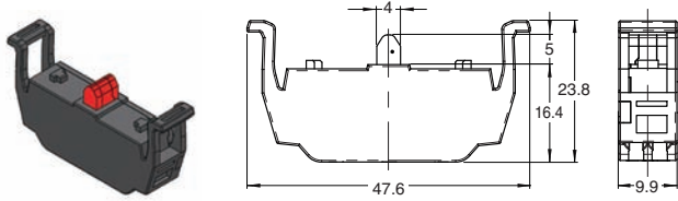
Switch Block (one contact) A22NZ-S-P1□N
