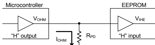
Figure 50. Pull down resistance
