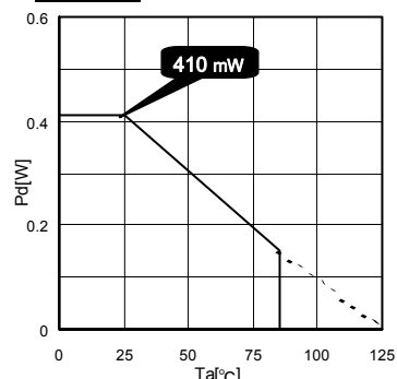
Fig.27 HVSO5 Power Dissipation vs Heat Reduction (Example)
