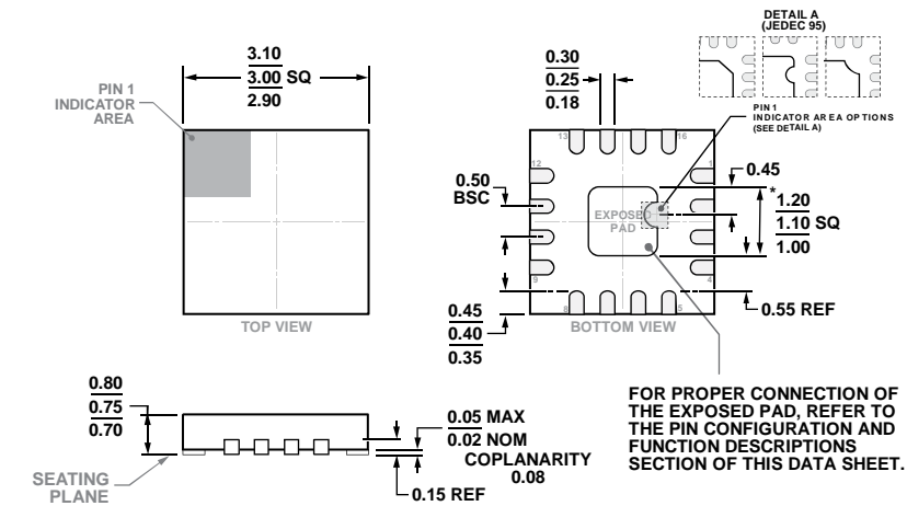
Figure 46. 16-Lead Lead Frame Chip Scale Package [LFCS] 3 mm x 3 mm Body and 0.75 mm Package Height (CP-16-45) Dimensions shown in millimeters
