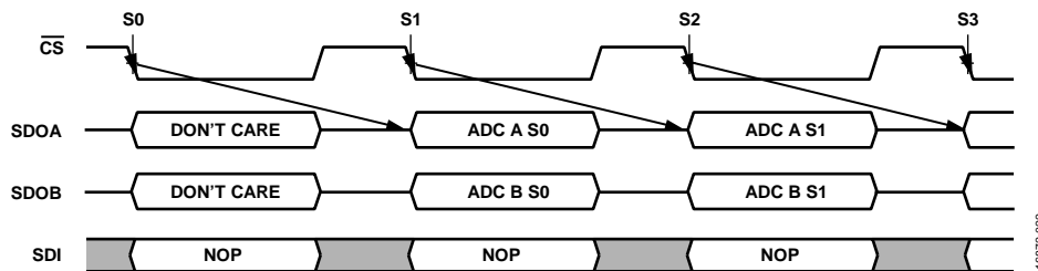
Figure 40. Reading Conversion Results for 2-Wire Mode
