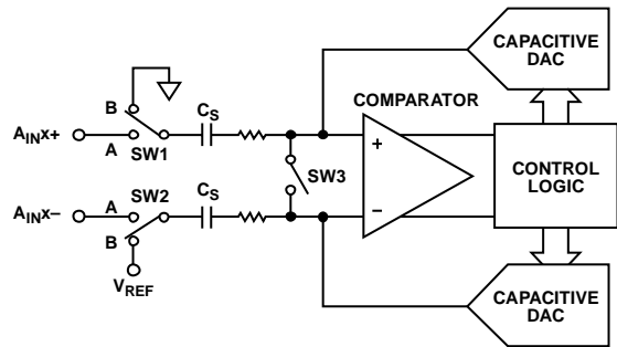
Figure 30. ADC Conversion Phase
