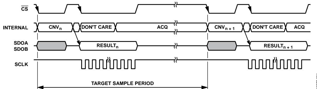
Figure 42. Low Throughput Low Latency
