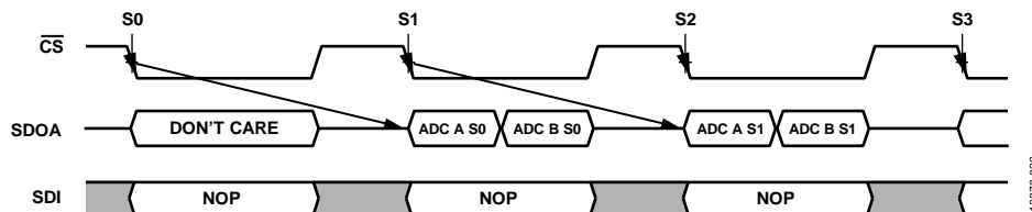
Figure 41. Reading Conversion Results for 1-Wire Mode
