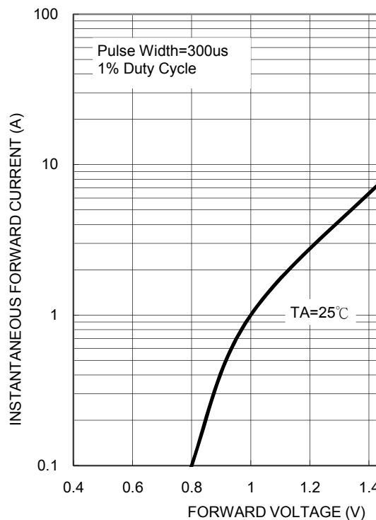
FIG. 5 TYPICAL FORWARD CHARACTERISTICS
