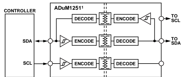
Figure 69. Isolated Interface
