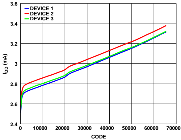
Figure 36. I_{DD} vs. Code
