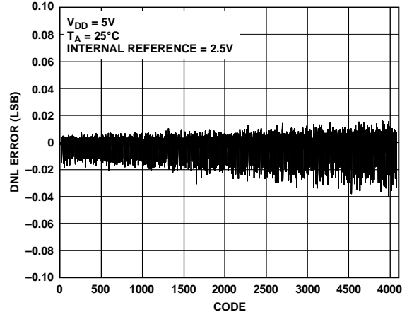
Figure 10. AD5674/AD5674R DNL Error vs. Code
