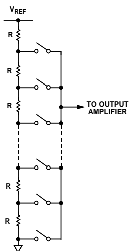
Figure 58. Resistor String Structure
