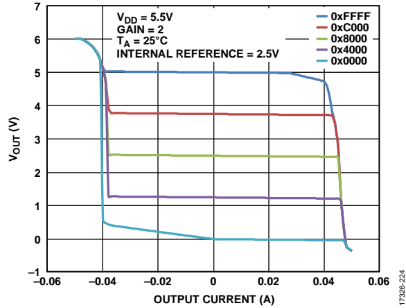
Figure 37. Source and Sink Capability at V_{DD} = 5.5V
