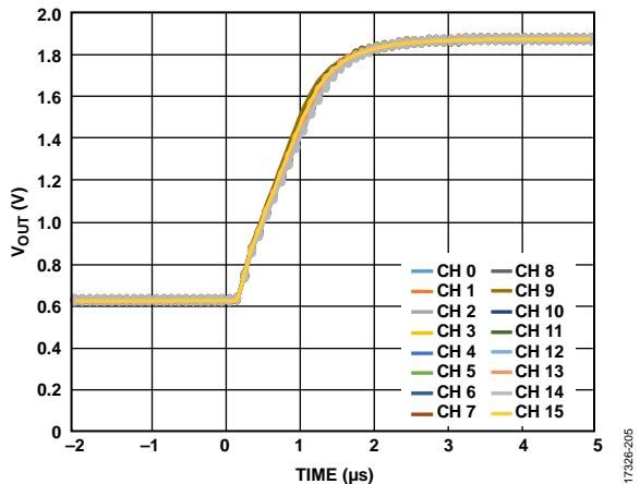
Figure 42. Settling Time
