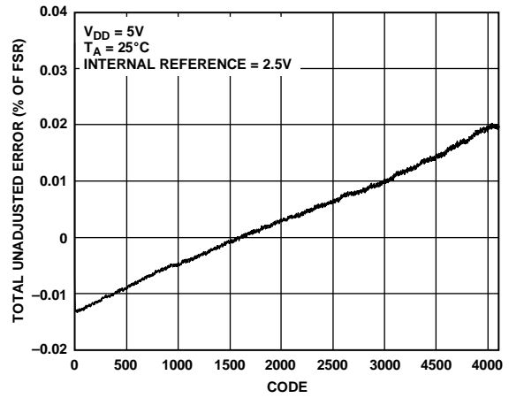
Figure 12. AD5674/AD5674R Total Unadjusted Error vs. Code
