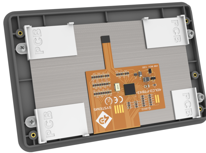
4DLCD-FT843 Mounted in 4.3" Bezel - Back
