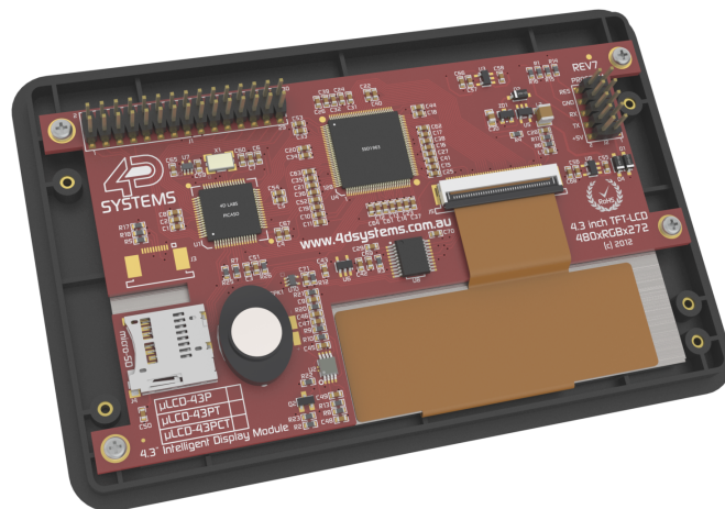
uLCD-43PT Mounted in 4.3" Bezel - Back
