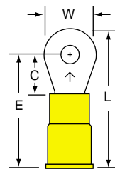
MVU10-6R Stud Size 6 Wire Range 12-10
