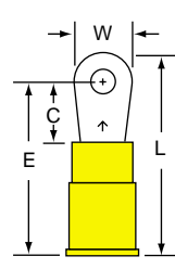
MVU10-4R/S Stud Size 4 Wire Range 12-10
