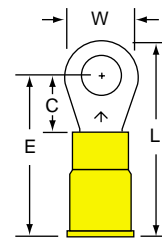
MVU10-10R Stud Size 10 Wire Range 12-10
