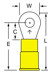
MVU10-8R Stud Size 8 Wire Range 12-10
