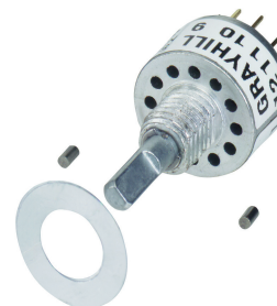
Adjustable Stop
