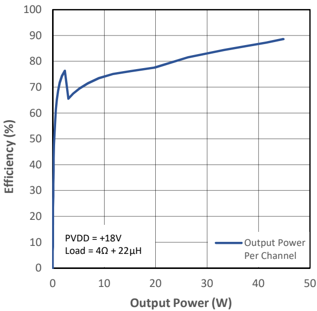
Figure 10-11 PMP2 Efficiency (VDD+PVDD) vs Output Power
