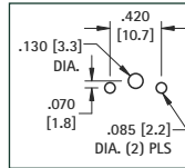
Mounting Detail
