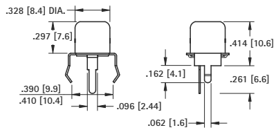
Mounting Detail
