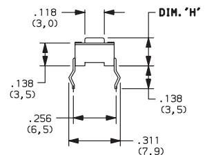
PTS635SL43 SPST
