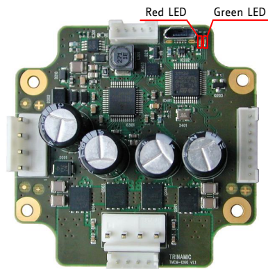
Figure 2: PD57/60/86-x-1260 LEDs
