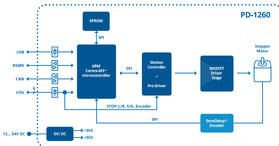
Figure 22: PD57/60/86-x-1260 block diagram
