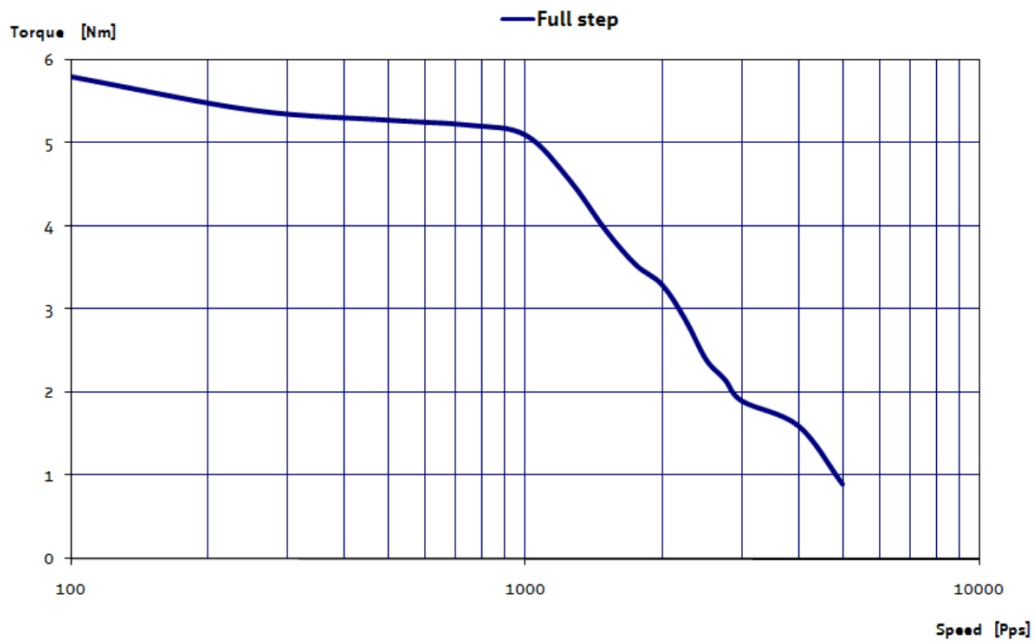
Figure 21: PD86-3-1260 torque vs. velocity 48V / 5.5A, full step operation
