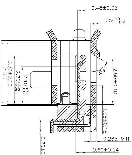
SECTION "A-A" (2:1)
