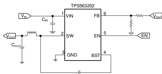
Copyright © 2019, Texas Instruments Incorporated 简化版原理图
