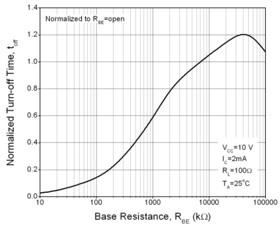
Figure 10. Turn-off Time vs Base-Emmitter Resistance
