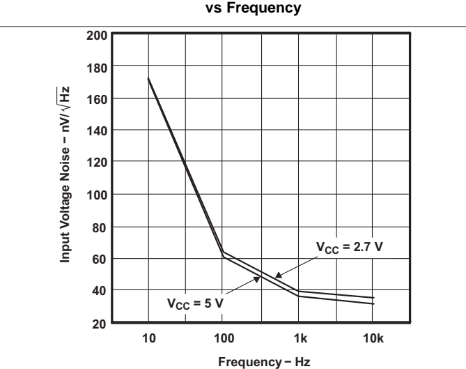
Figure 36. Input Voltage Noise vs Frequency
