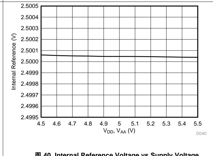
图 40. Internal Reference Voltage vs Supply Voltage
