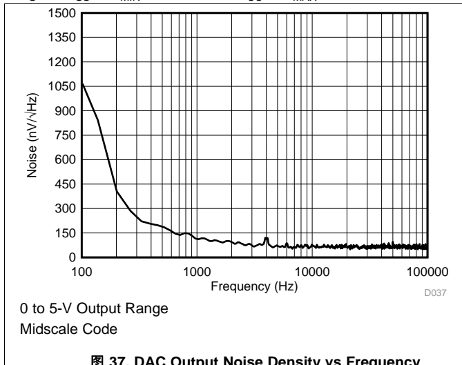
图 37. DAC Output Noise Density vs Frequency
