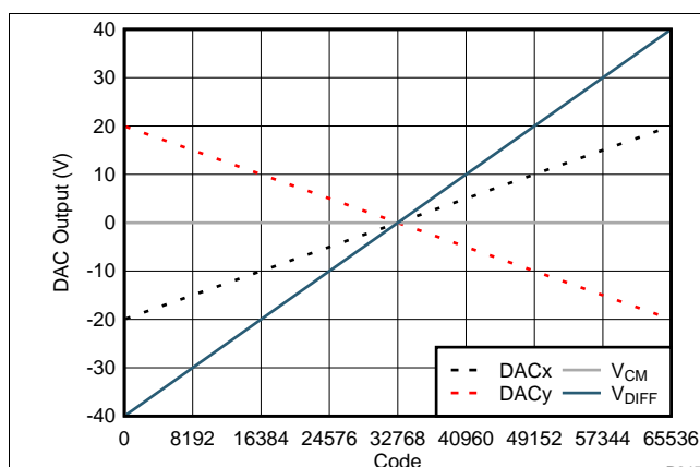
图 48. Differential Bipolar Output (16-Bit): \pm 20 -V Output Range
