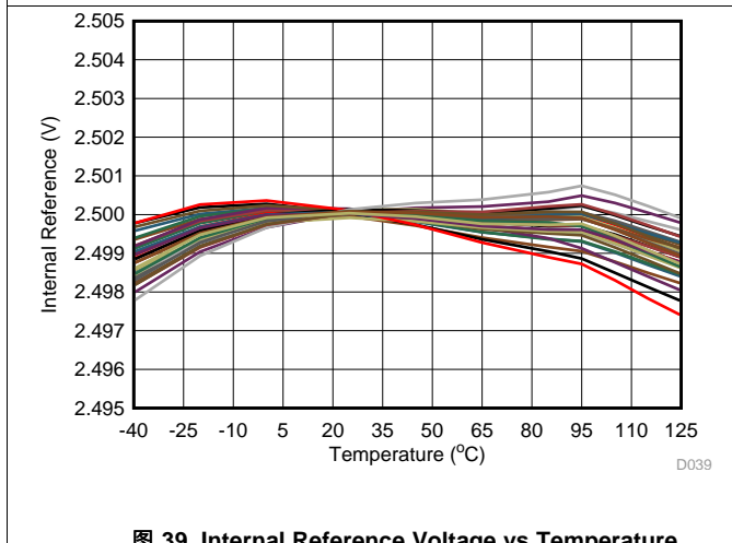
图 39. Internal Reference Voltage vs Temperature
