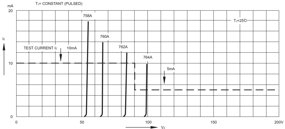
FIG.11- BREAKDOWN CHARACTERISTICS
