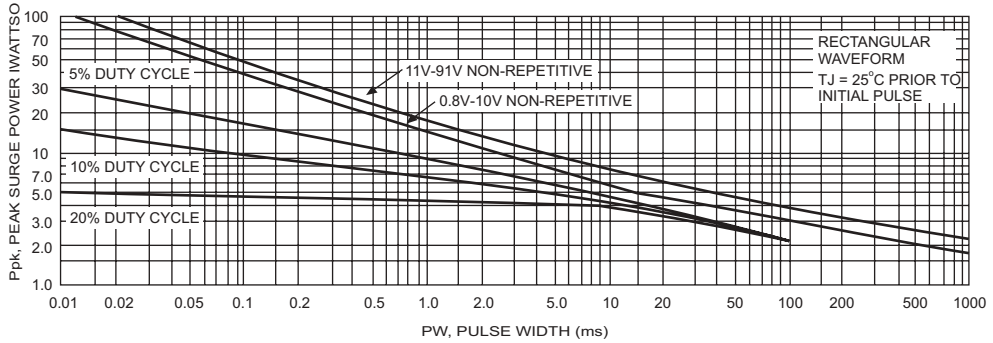
FIG.10- BREAKDOWN CHARACTERISTICS
