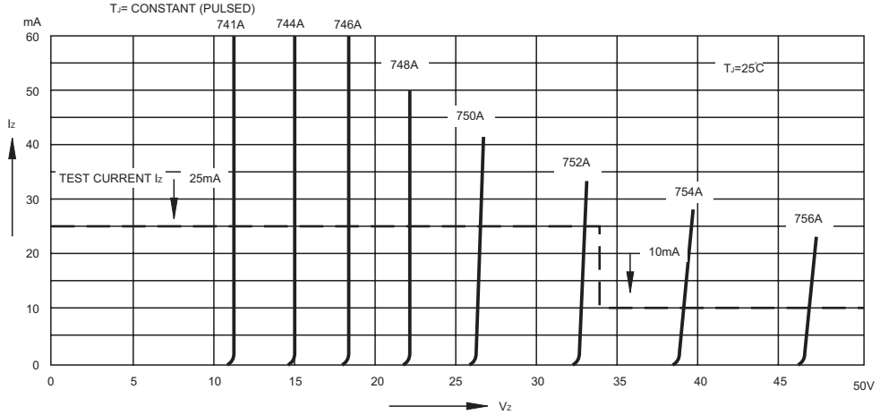
FIG.11- BREAKDOWN CHARACTERISTICS
