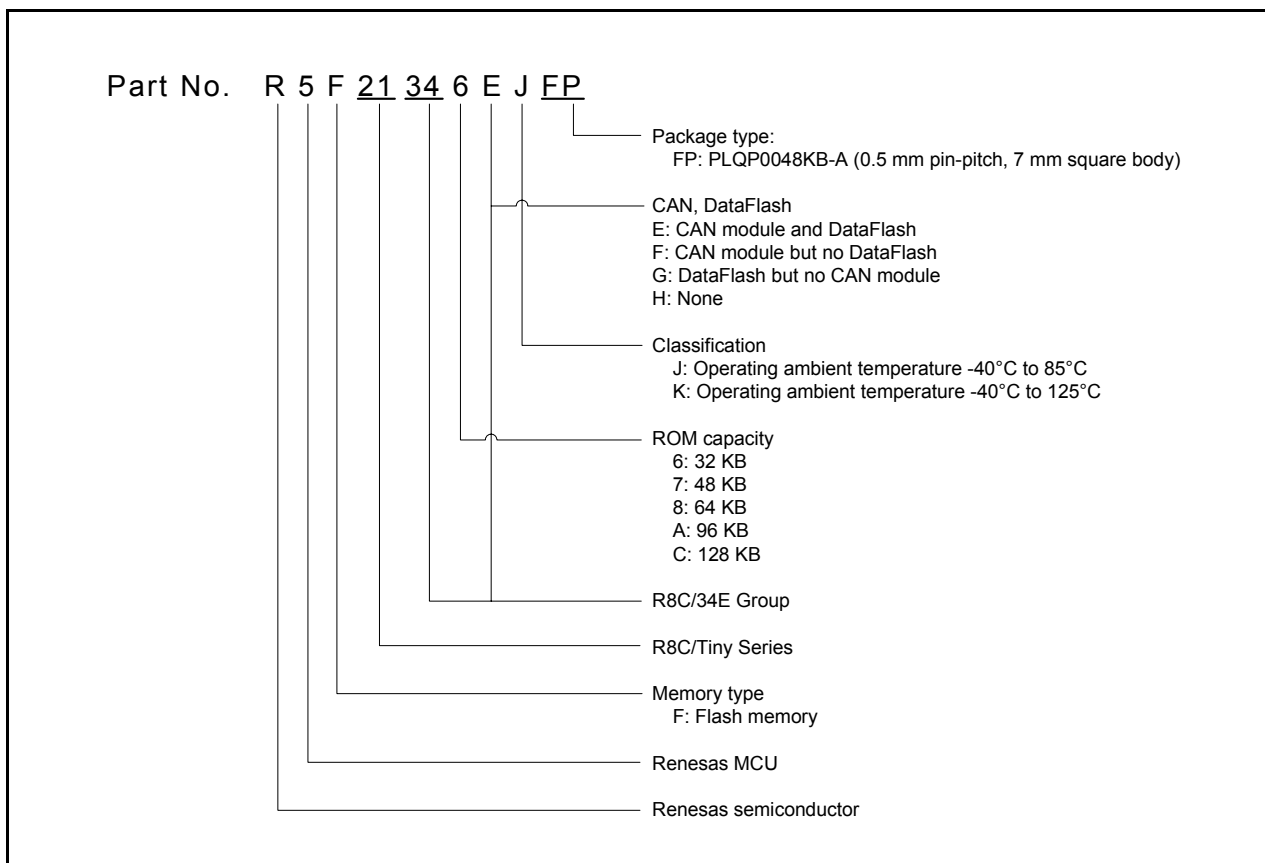
Figure 1.1 Part Number, Memory Size, and Package of R8C/34E Group
