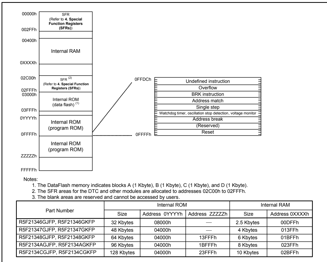
Figure 3.3 Memory Map of R8C/34G Group
