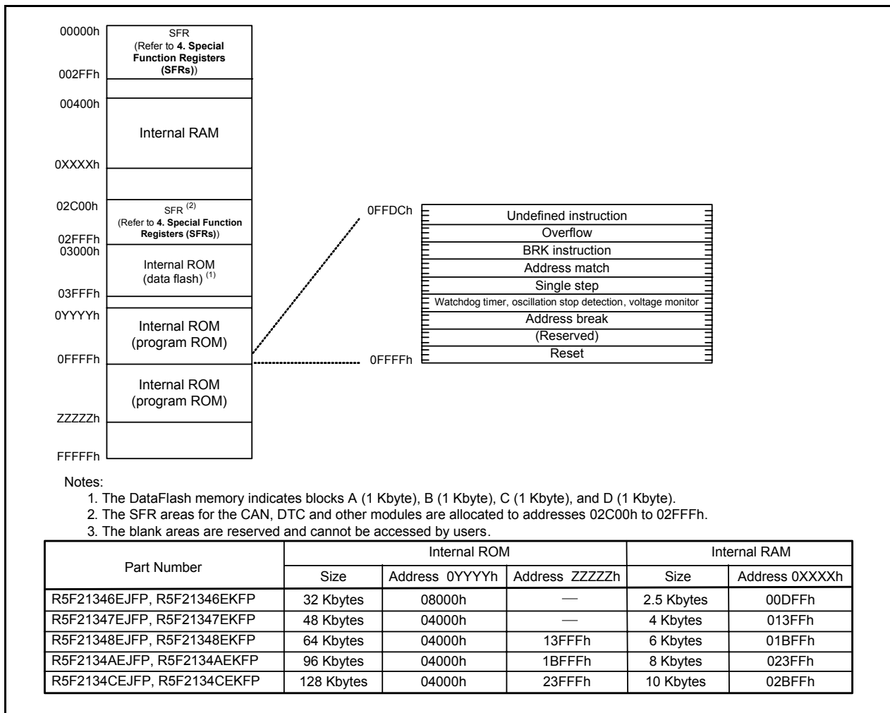
Figure 3.1 Memory Map of R8C/34E Group
