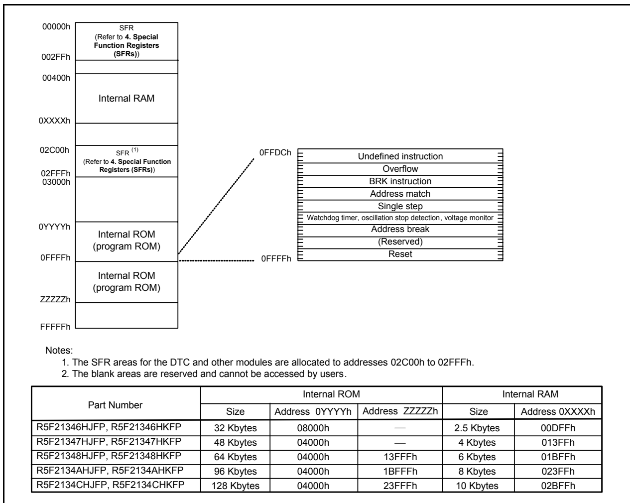
Figure 3.4 Memory Map of R8C/34H Group
