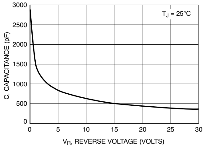
Figure 7. Typical Capacitance for MBR30H30CTG
