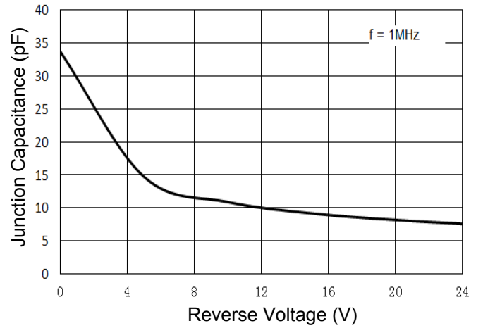
Fig 4. Junction Capacitance
