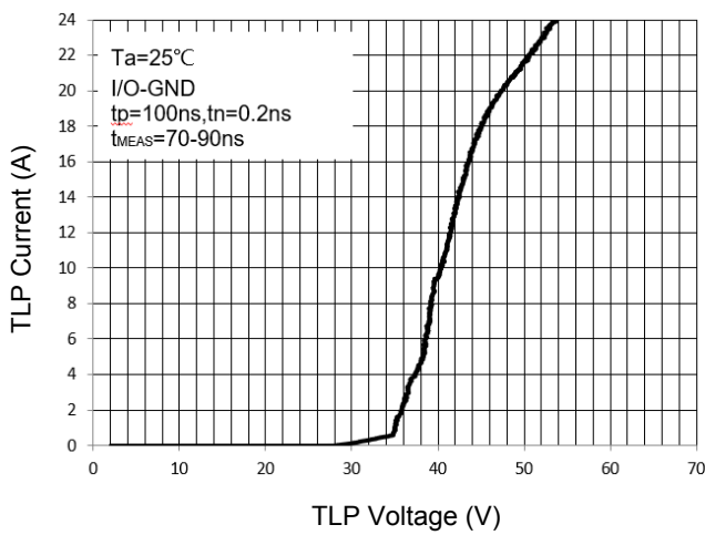
Fig 5 TLP Curve
