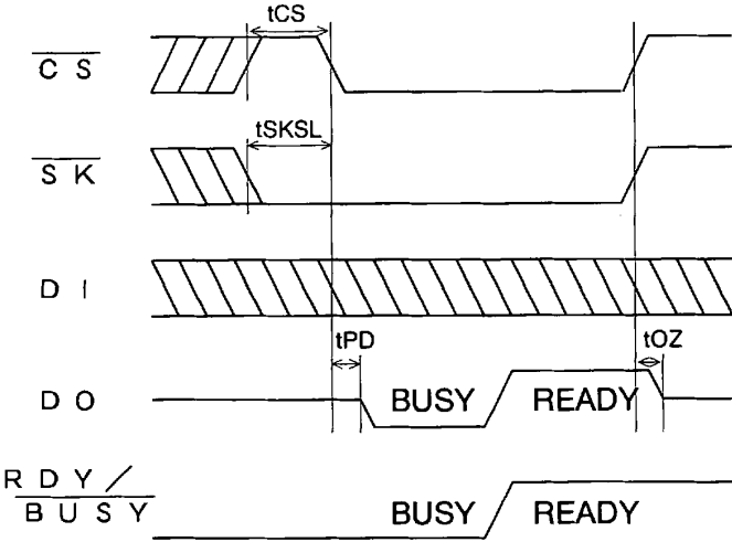
Ready / \overline{BUSY} Signal Output ( DO pin )
